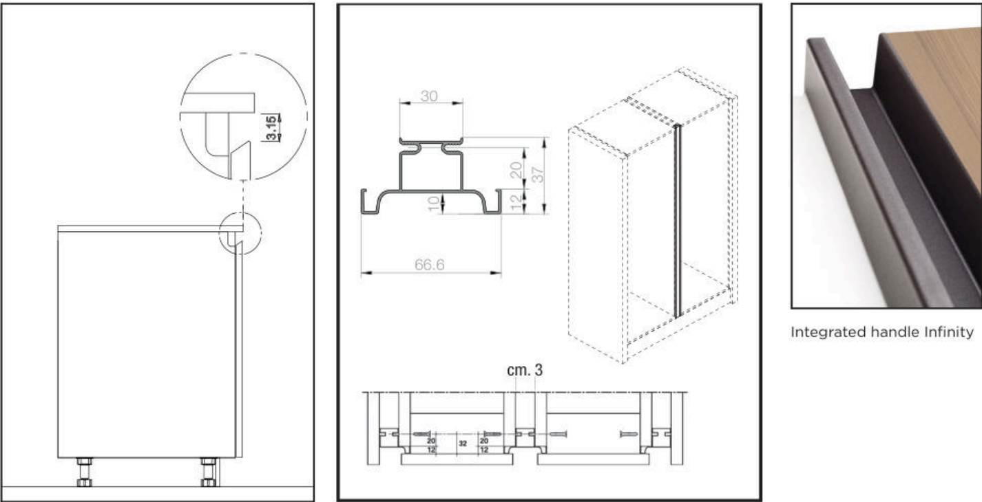
Flat channel + 35° cut
